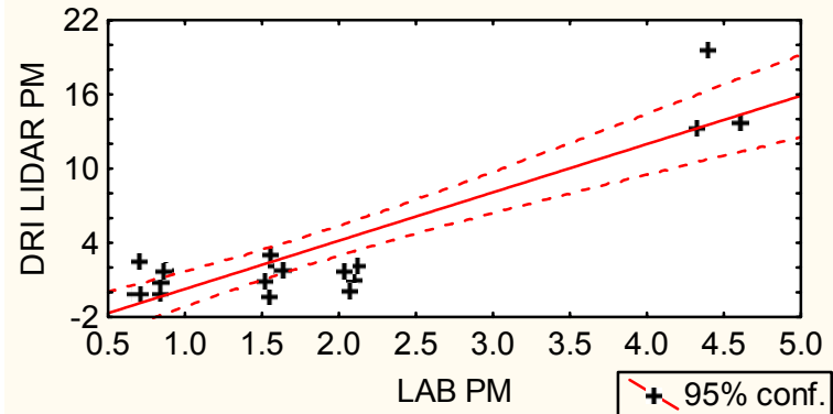
Scatterplot: LAB PM vs. DRI LIDAR PM (Casewise MD deletion) Ramp DRI LIDAR PM gm/kg Fuel = -3.6 + 3.9 * \text{LAB PM} Correlation: r = 0.89
